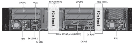
(2)DW-GPU+4PCIe
