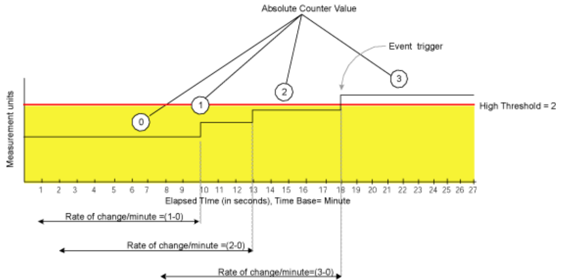
FIGURE 3 Event trigger
