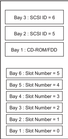
"Tower type's front view"
