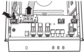
[Top view of operator panel]
