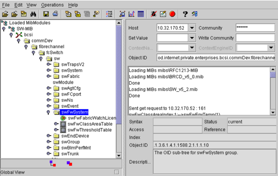
FIGURE 6 Example OID tree
