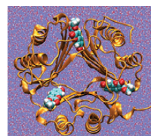
Snapshot of protein (MIF)-ligand complex in solvent
