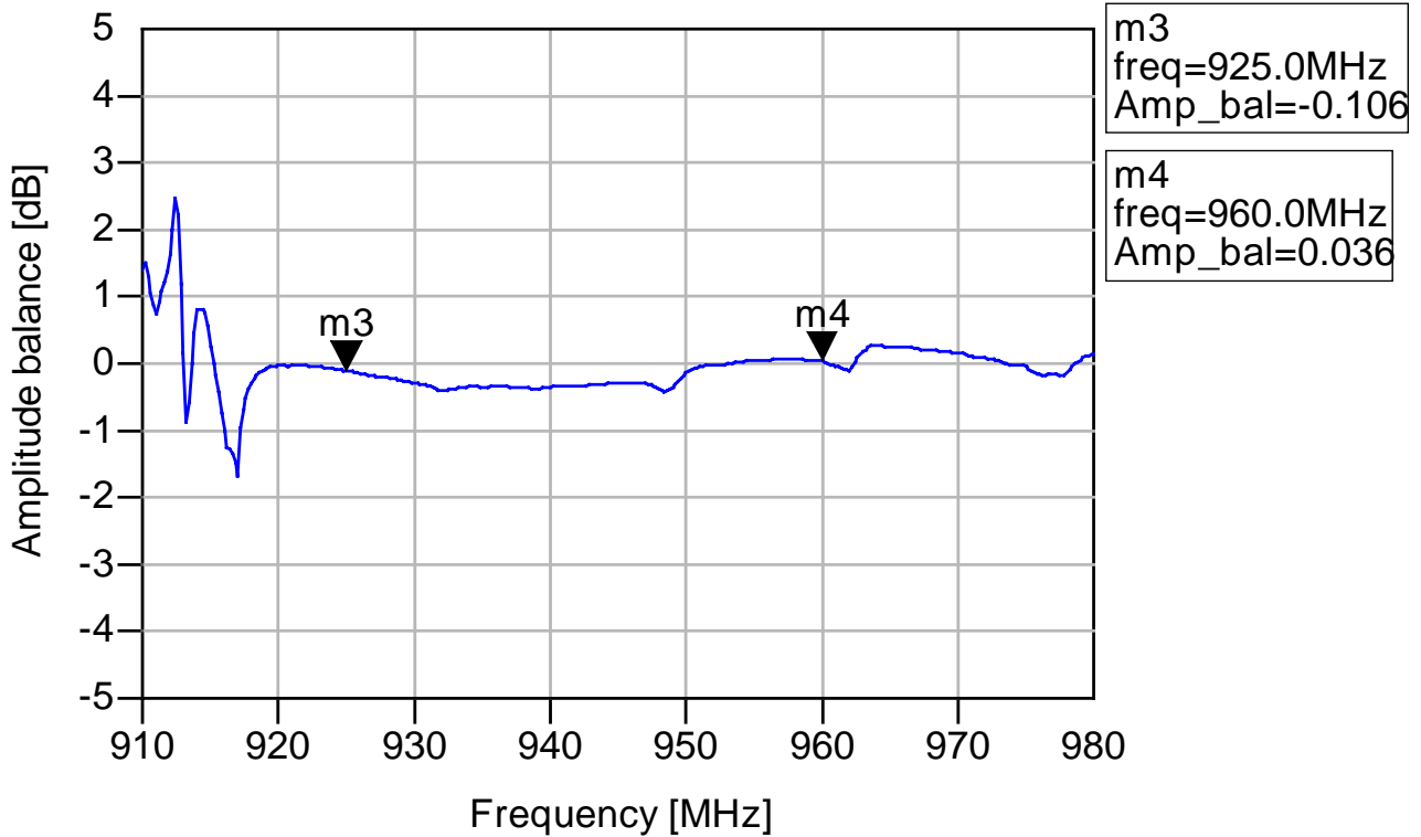
Fig.7 Amplitude balance
