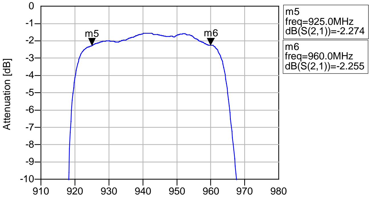
Frequency [MHz] Fig.3 In-band Characteristics
