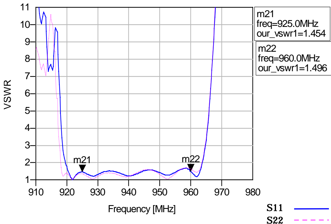
Fig.2 VSWR
