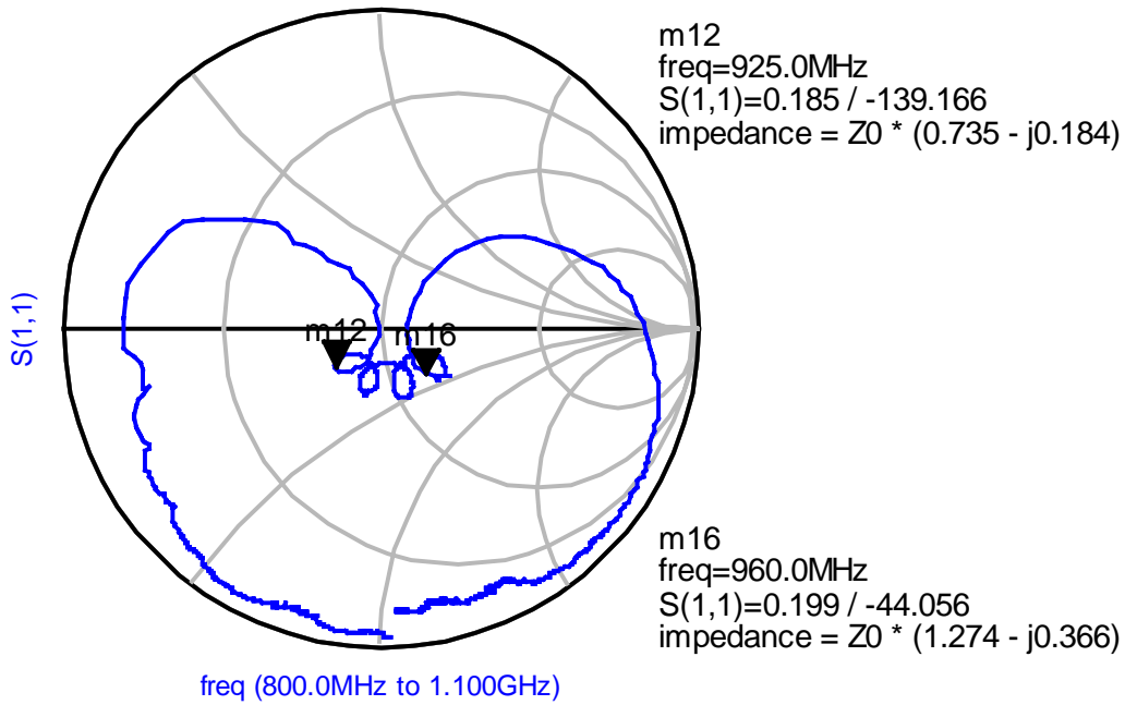
Fig.5 S11
