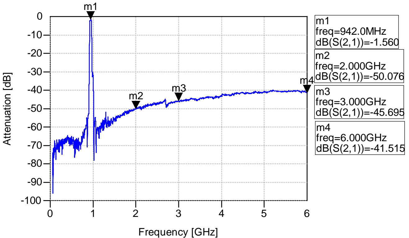
Frequency [GHz] Fig.4 Wide-band Characteristics
