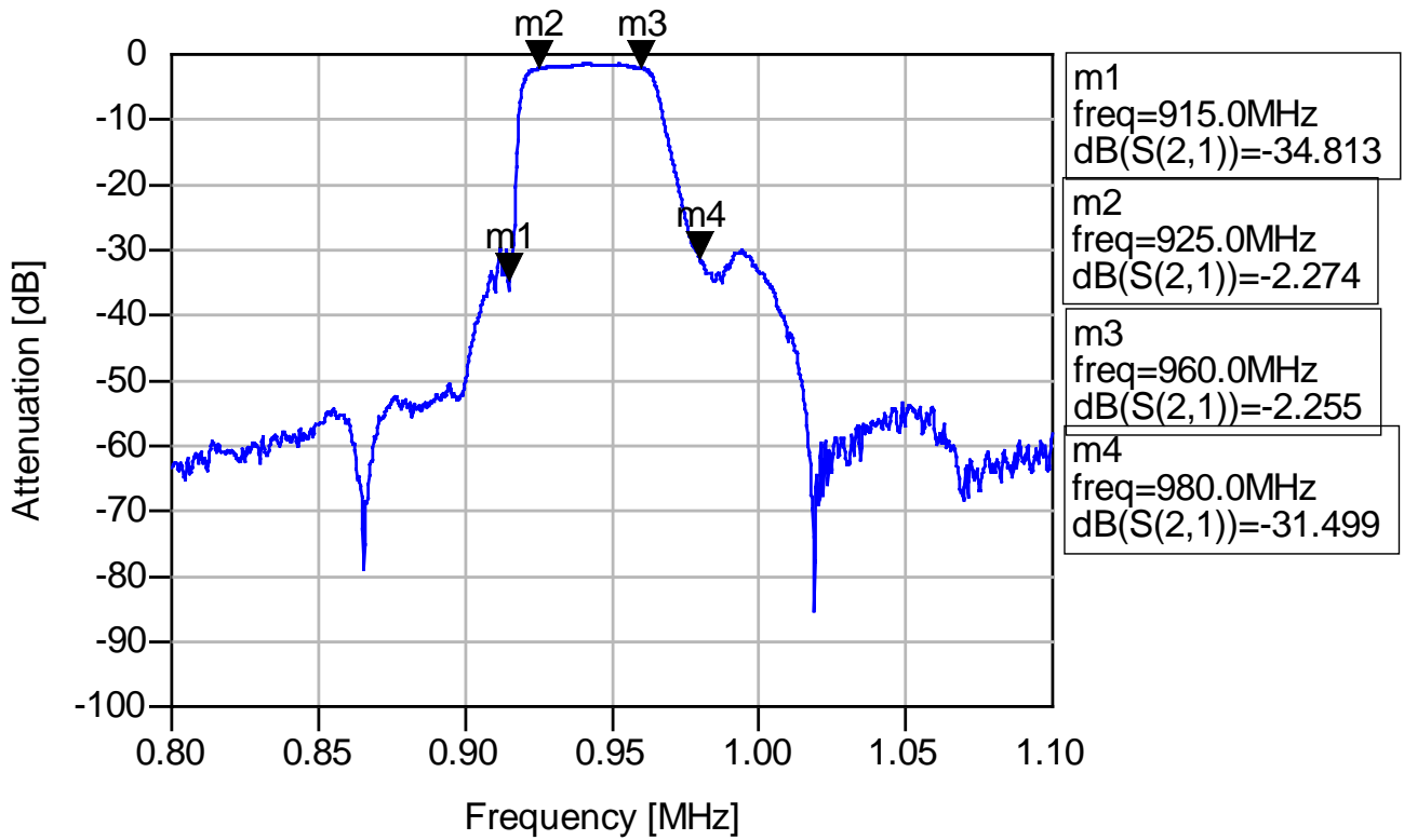
Fig.1 Pass-band Characteristics
