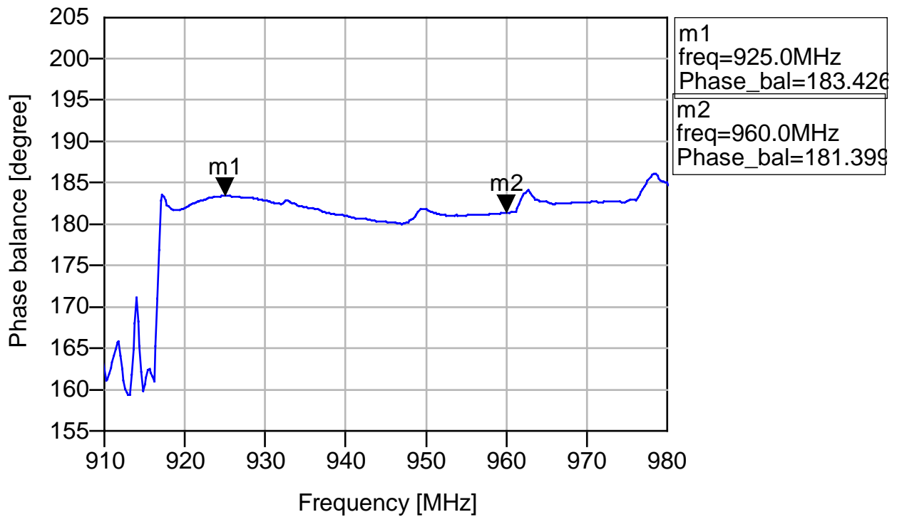
Fig.8 Phase balance
