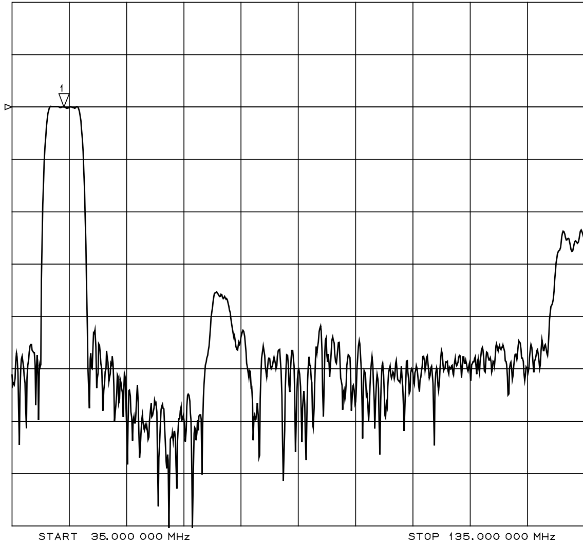
Amplitude Response (10dB/div) ( 35.0MHz ----- 135.0MHz )
