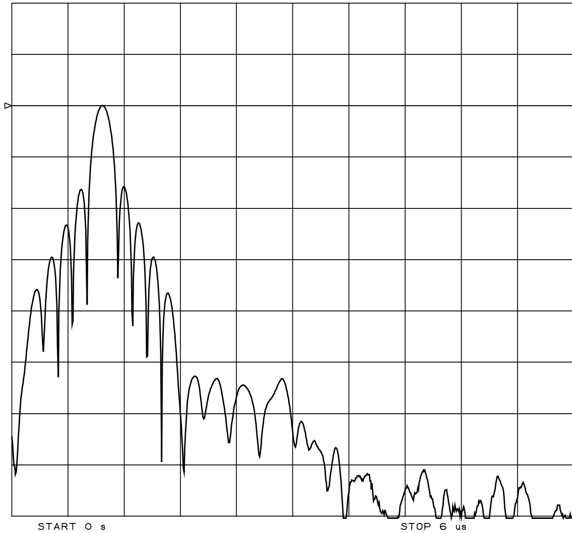
Time domain Response (10dB/div)
